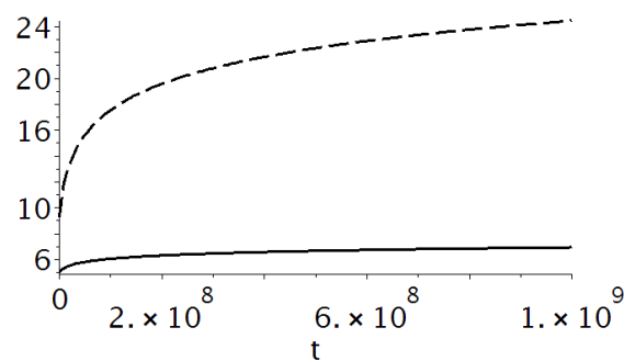
Figure 2. Time dependence of the size of extra space (solid line) and the main 4-dimensional space (dashed line) in a logarithmic scale; extra dimension, n = 5 , the D -dimensional cosmological constant, \Lambda_D = 0.0125 .
