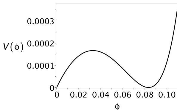
Figure 1. The effective potential for a viable version of the model (1). The minimum of the potential is at the point \phi_{\min} \simeq 0.083 , the D -dimensional Planck mass, m_D = 1 . In agreement with [24], m_D \sim 0.1 M_{Pl} , where M_{Pl} is the Planck mass.
