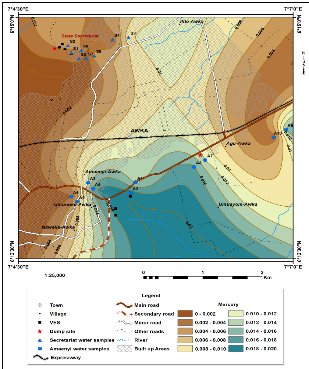
Fig. 7. Distribution of mercury in the study area
