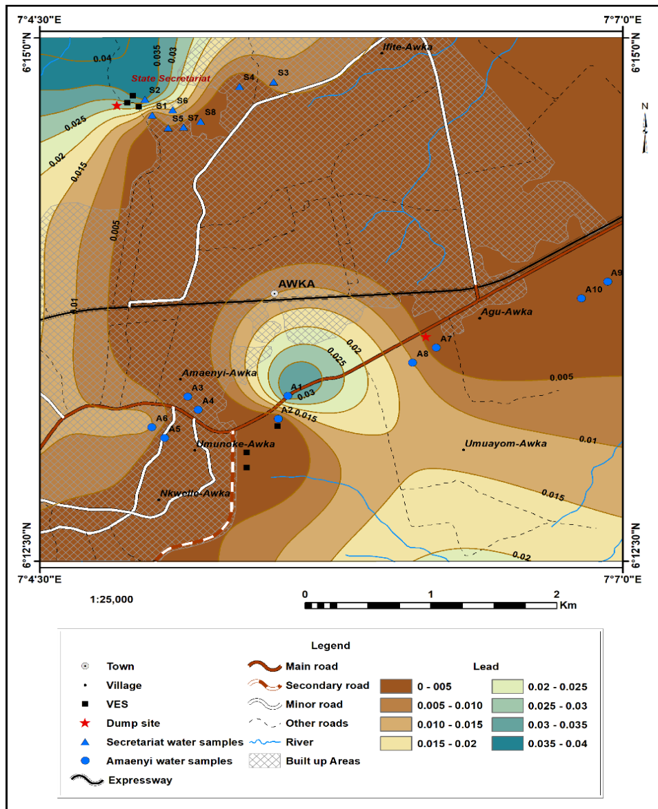
Fig. 8. The spatial distribution of lead in the study area
