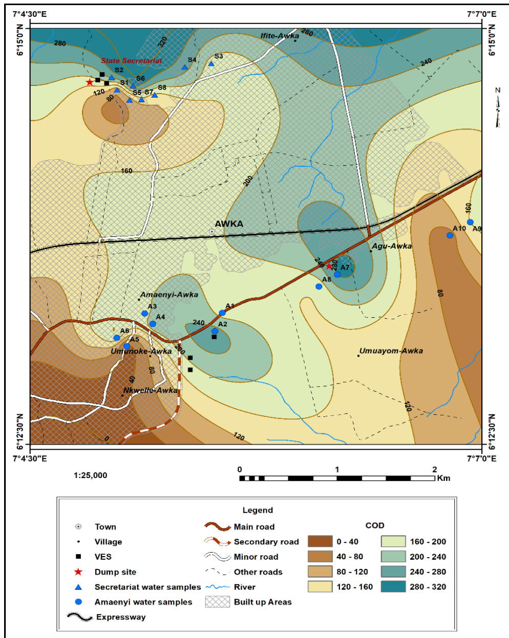
Fig. 4. The spatial distribution of COD in the study area
