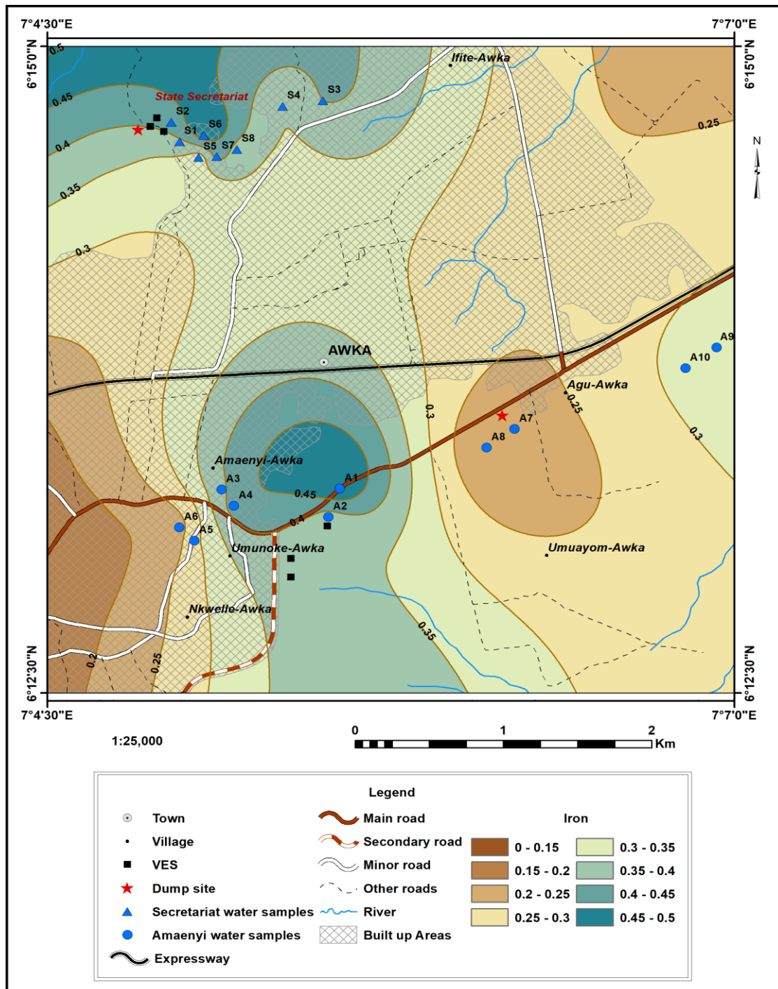
Fig. 5. The distribution of the concentration of iron in the study area
