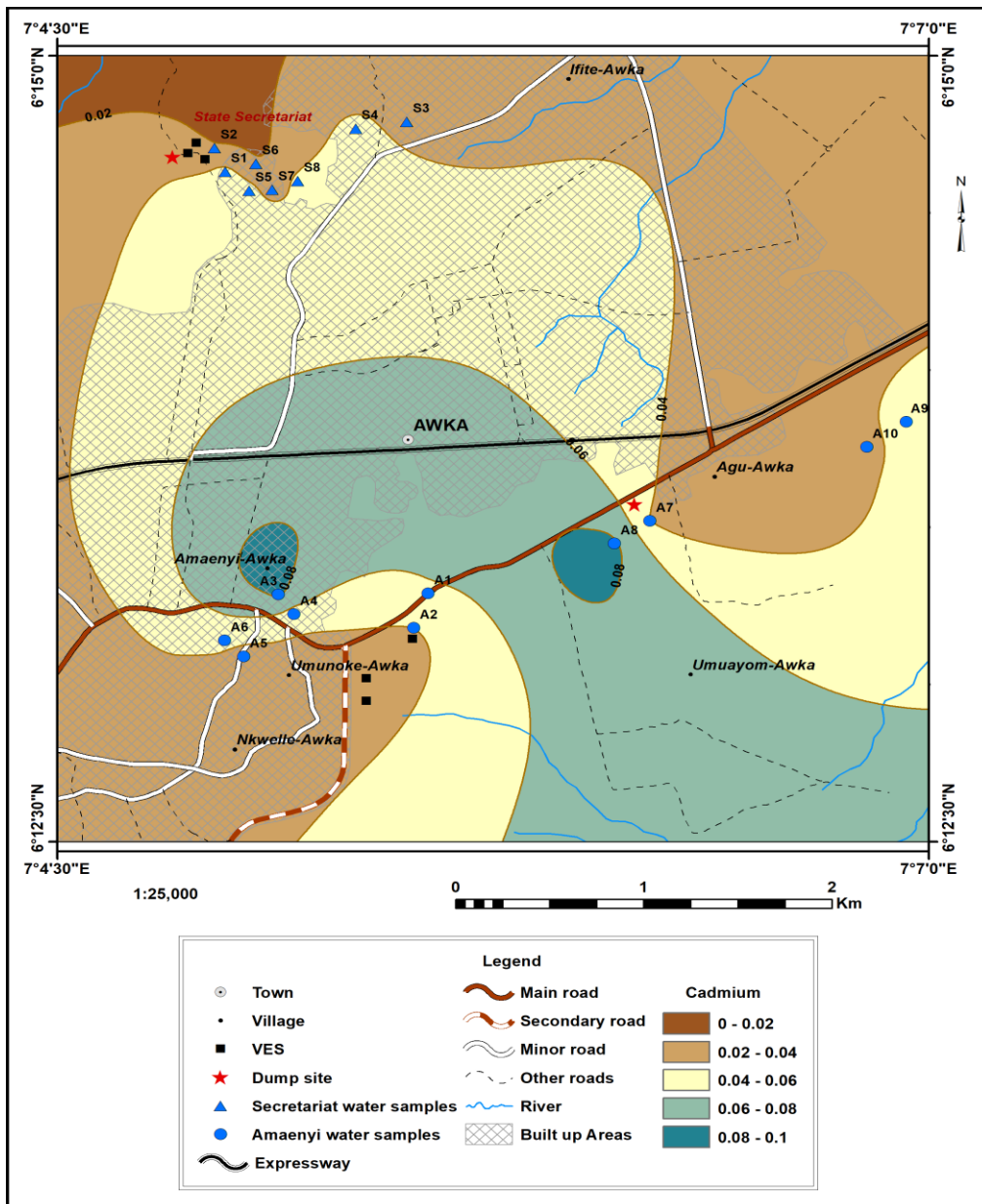
Fig. 6. The distribution of cadmium in the study area
