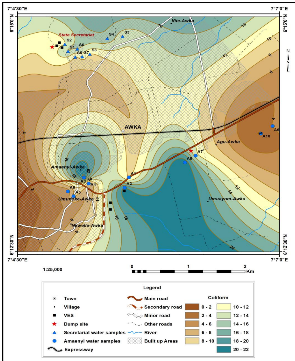
Fig. 11. The distribution of coliform bacteria in the study area
