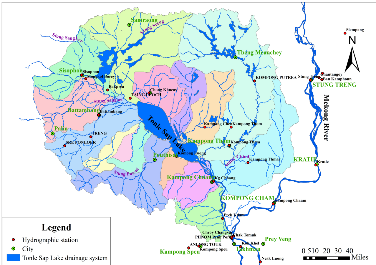
Figure 1. Water system map of Tonle Sap Lake basin.
