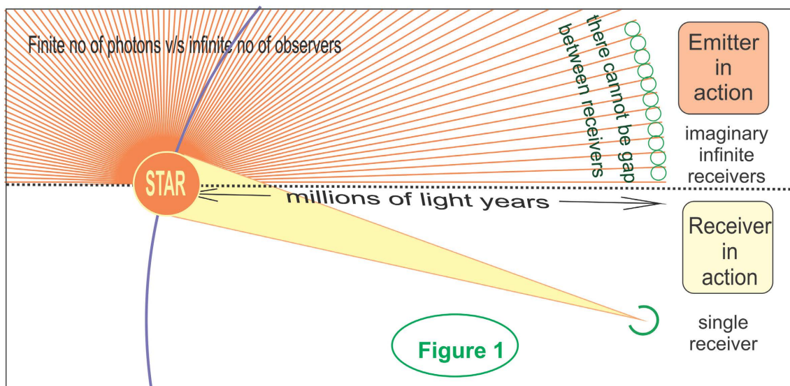
Figure 1. Emission of photons: An emitter can have infinite receivers. The Sun can be seen from infinite positions. If the Sun throws light, it must throw light in infinite directions, which is never possible. Here, the word infinite is used only for infinity, not just for a large number. Any emitter, however large, cannot have infinite photons. This logic proves that the emitter does not throw photons.
