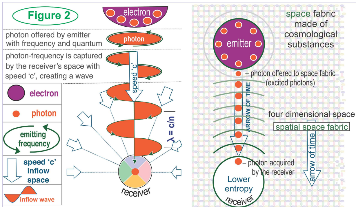
Figure 2. Propagation of light: The emitter consists of a higher entropy zone that comprises quantum and frequency. The receiver consists of a lower entropy zone that comprises direction and speed. The lower entropy of the receiver evolves an arrow of time, whose direction is toward the receiver itself. In other words, the receiver is responsible for carrying photons. The receiver captures the quantum and frequency, amalgamates with direction and speed, and creates an electromagnetic wave. All these functions occur at the space fabric, which is made of systematically arranged energy fields.
