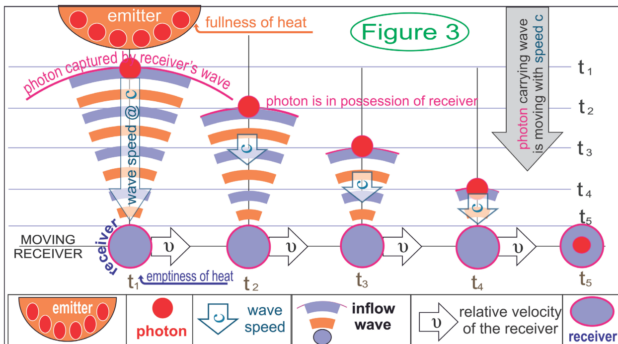
Figure 3. The emitter with the fullness of heat departs the photon, where the inflowing wave of the receiver captures it for acquisition. Subsequently, no connection exists between the emitter and photon. The receiver lying in the lower entropy zone creates an arrow of time toward itself. Once the receiver's wave captures the photon, it remains within the wave till it reaches the acquiring receiver. While measuring the speed of light, we measure only the inflow wave speed of the receiver, which has no connection to the emitter.
