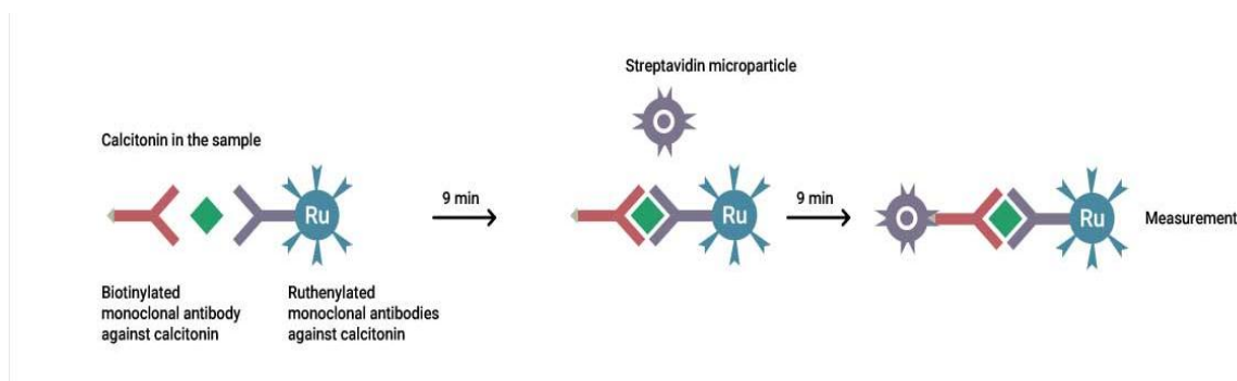
Fig. 1. Electrochemiluminescence immunoassay
