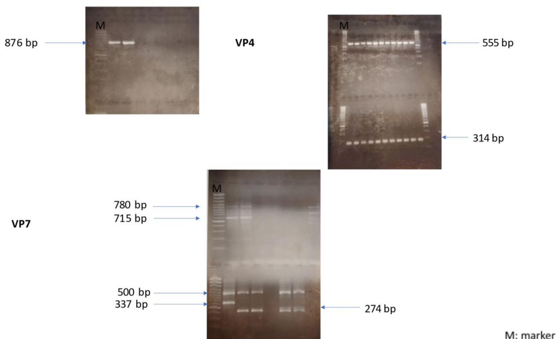
Fig. 1. Detection of Calves and Piglets rotavirus by RT-PCR
