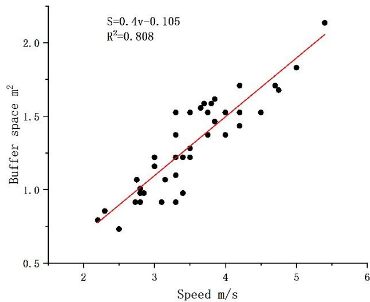
Fig. 7. Speed-buffer space model in running state
