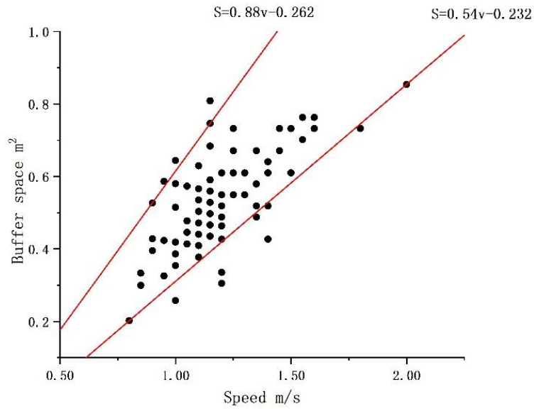
Fig. 6. Speed-buffer space model under normal motion
