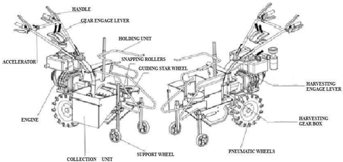
Fig. 1. Component of maize cob harvester
