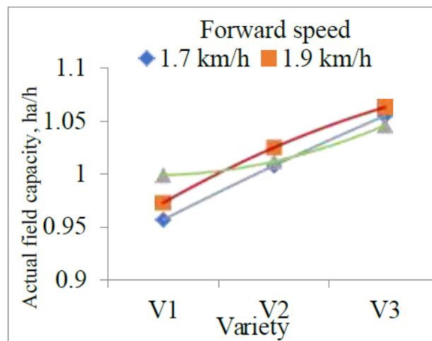
Fig. 10. Effect of forward speed and variety on actual field capacity by maize cob harvester
