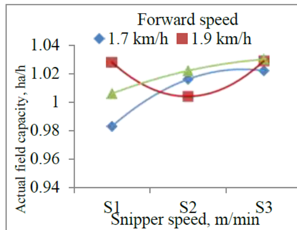
Fig. 9. Effect of forward speed and sniper speed on actual field capacity by maize cob harvester
