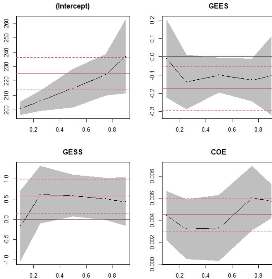
Fig. 3. Plots of the Coefficient Estimates of the Explanatory Variables with 95% band
