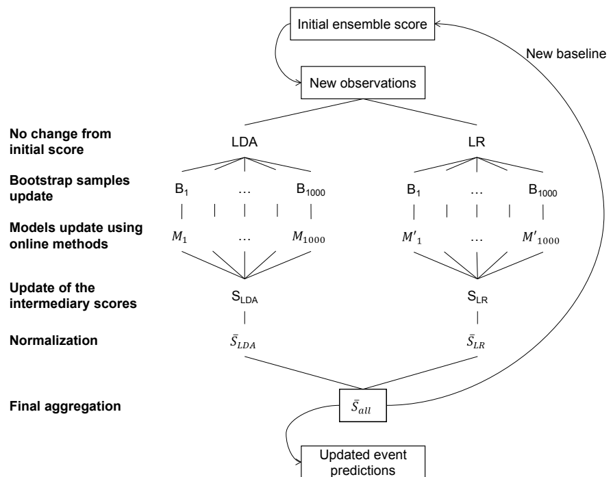
Figure 1. Methodology of construction and update of the online ensemble score.
