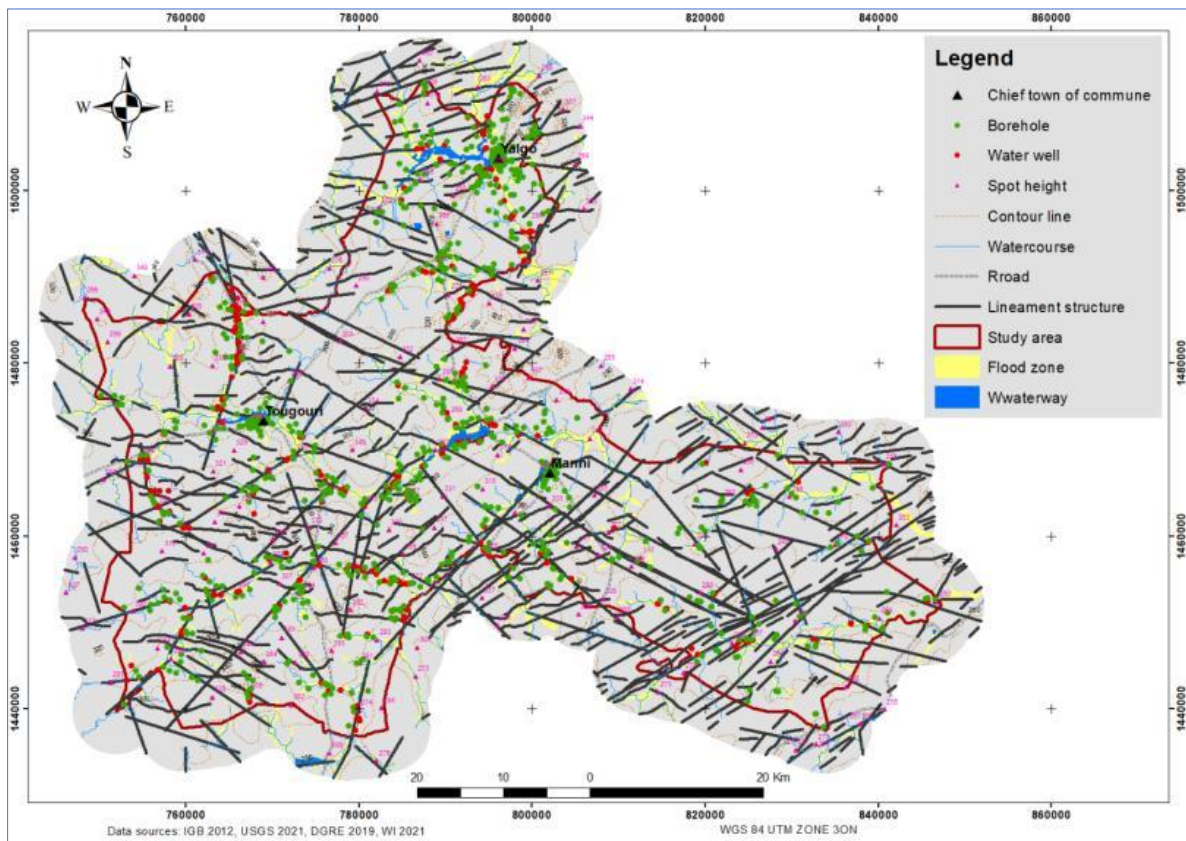
Fig. 5. Lineament structural map
