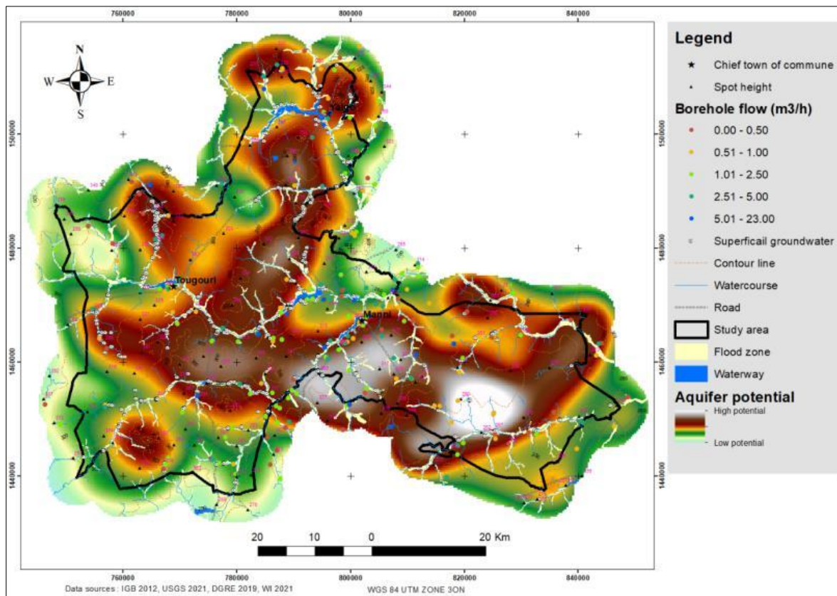
Fig. 7. Mapping of aquifer potential
