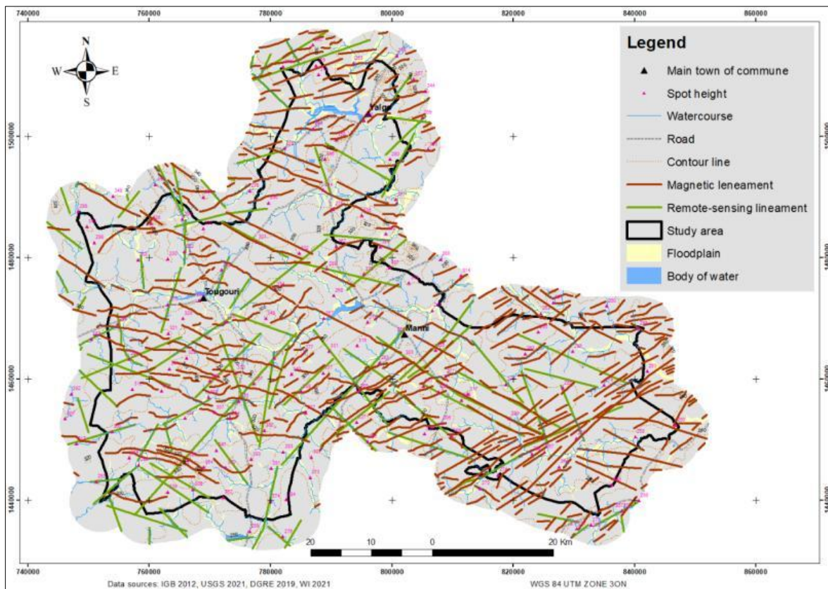
Fig. 3. Magnetic and remote-sensing lineament map
