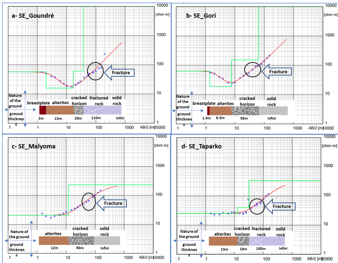
Fig. 4. Interpretation of electrical surveys
