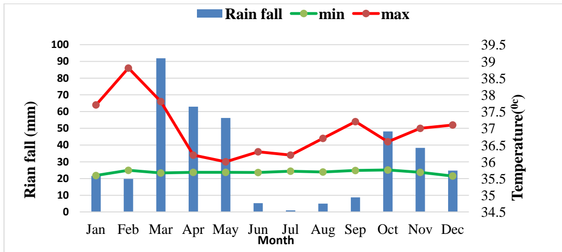
Fig. 2. Monthly rainfall, minimum and maximum temperature at Dasenech district (2000-2019 G.C)
